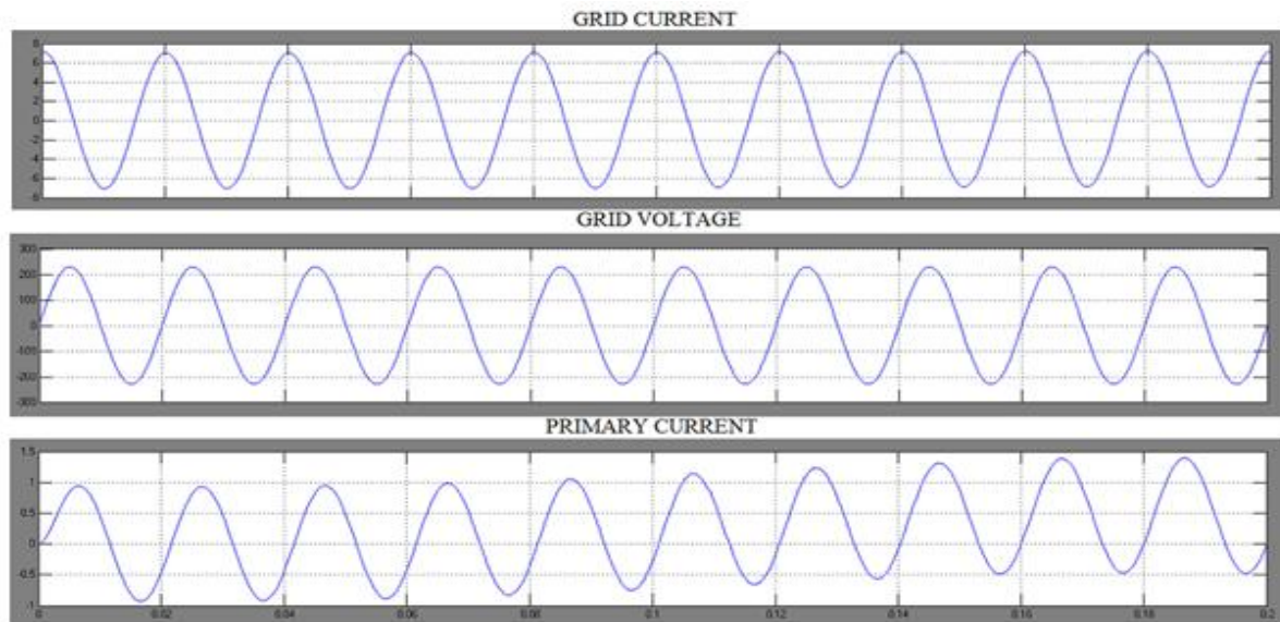
Figure 6: Output waveforms of Grid connected single-phase PV inverter with PRI controller.
