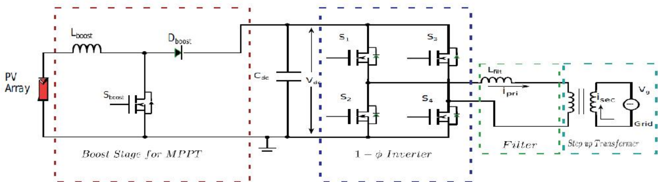
Figure 3: Power circuit topology of the 1 – phase PV system for a low-voltage inverter with 40V dc bus connected to 230V grid using a step-up transformer
