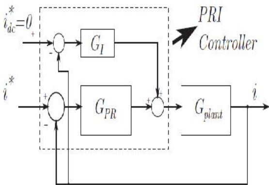
Figure 2: Block diagram of the fundamental current control with the PRI controller.
